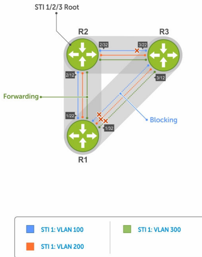
Figure 96. Per-VLAN Spanning Tree
